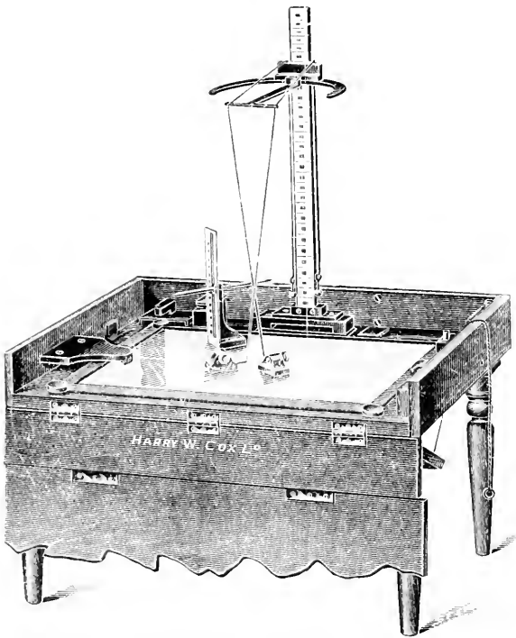
FIG. 93.—Mackenzie Davidson cross-thread localiser. (Cox and Co.).
